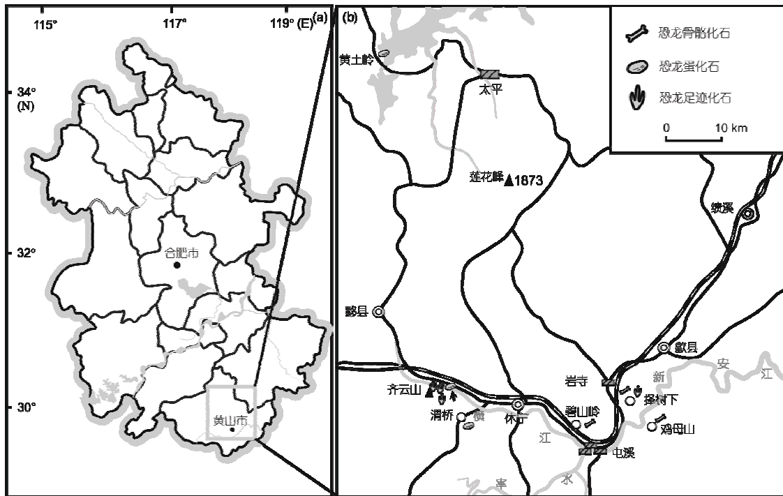
图1 皖南地区恐龙、恐龙蛋、恐龙足迹分布示意图(据余心起 [1] 修改). (b)中箭头所指为本文研究恐龙蛋的产出地点 Figure 1 Distribution map of dinosaur bones, dinosaur eggs, dinosaur footprints in South of Anhui (modified from Yu [1] ). The arrow shows the locality of dinosaur eggs in this paper in (b)
